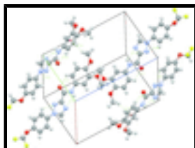
Fig. 2. CH- \pi interactions and \pi - \pi stacking interactions.
